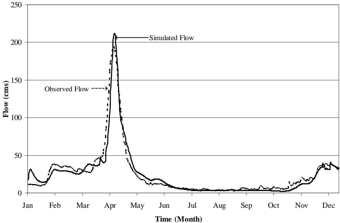
Simulated vs Observed Streamflow (1999) Mississippi River @ Appleton (WSC 02KF006)
