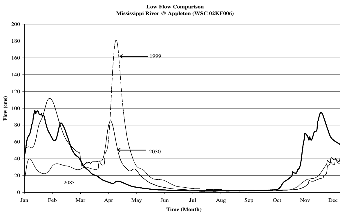
Figure 4.31. Low flow comparison for the Mississippi River at the Appleton gauge.
