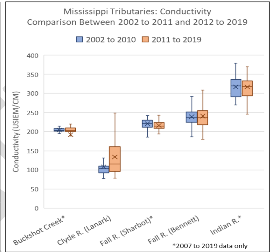
Figure 17: Mississippi Tributaries - Conductivity
