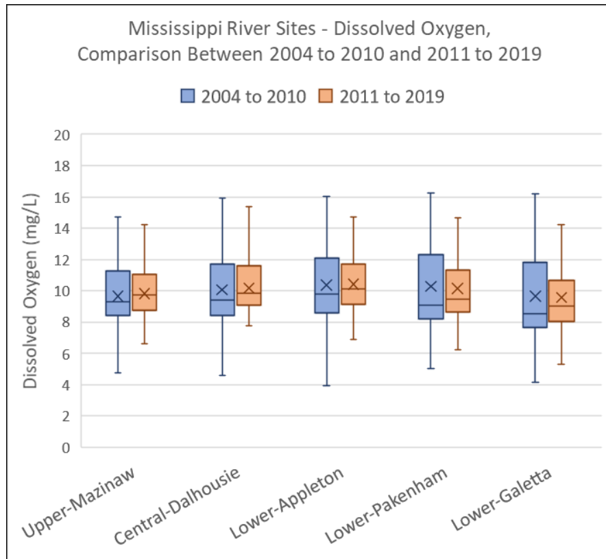
Figure 15: Mississippi River- Dissolved Oxygen
