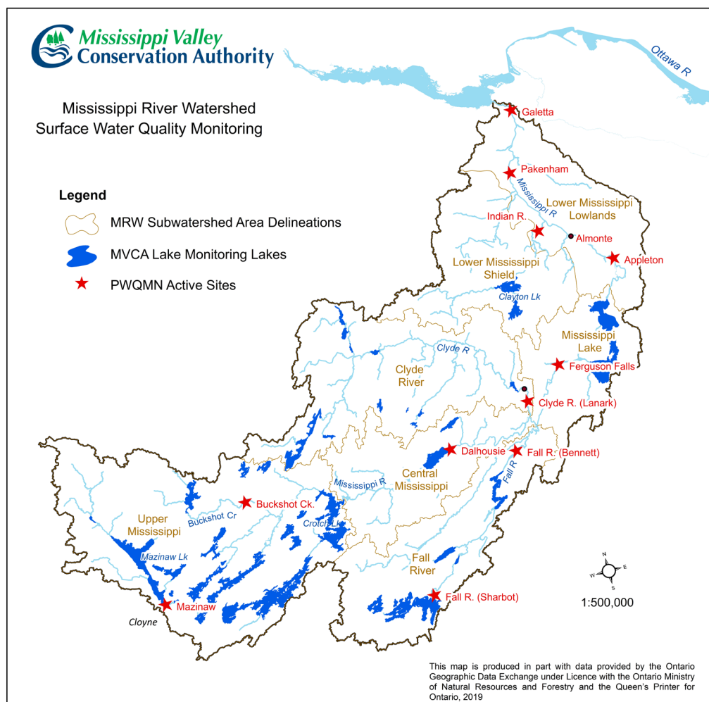
Figure 6: MVCA Lake Monitoring Sites and PWQMN Sites
