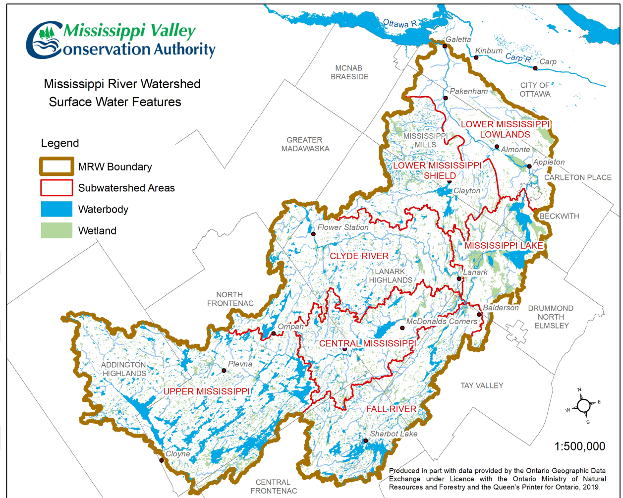
Figure 1: Mississippi River Watershed and Subwatersheds
