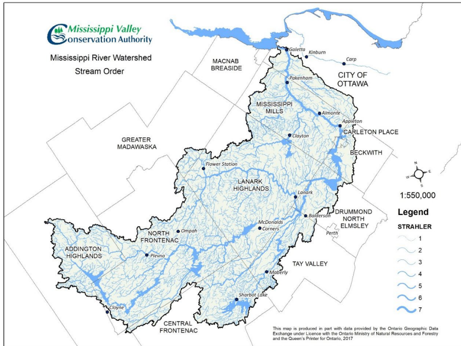
Figure 12: Mississippi Watershed Stream Order
