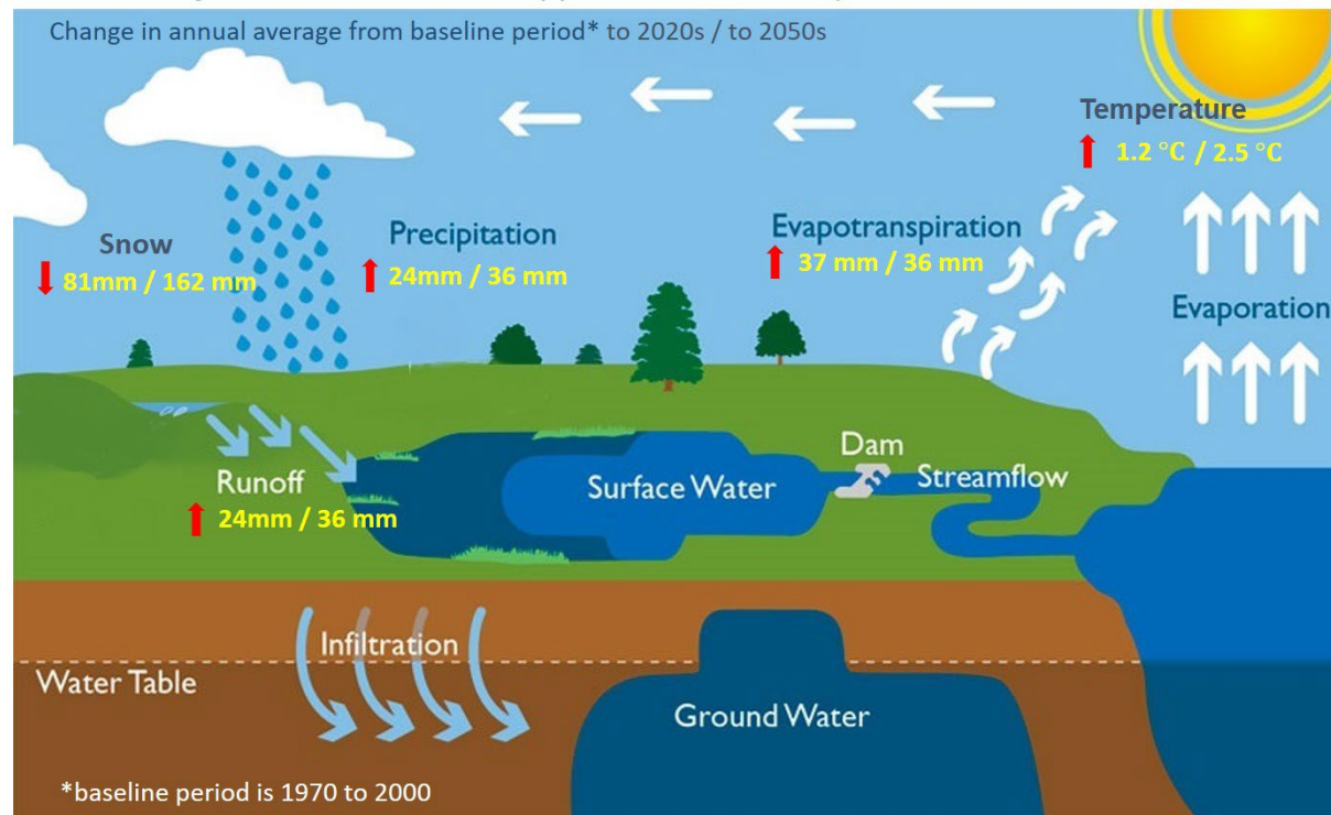
Figure 9: Projected Climate Change Impacts
