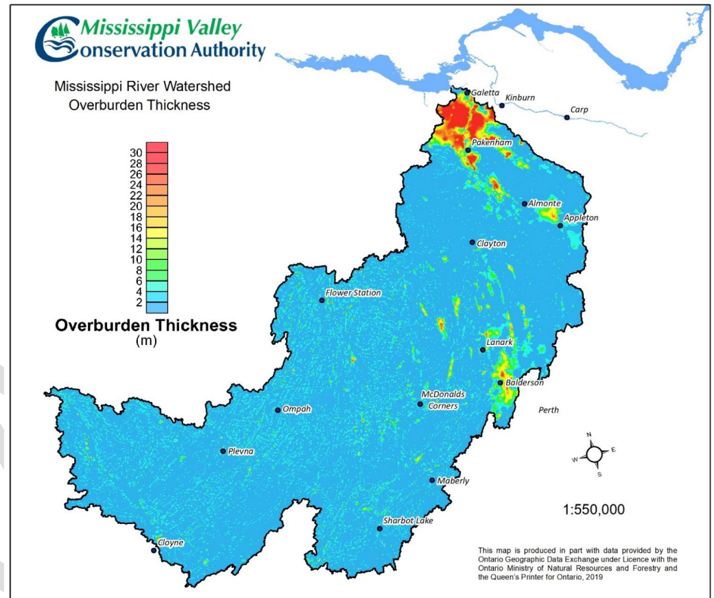
Figure 5: Interpreted Overburden Thickness
