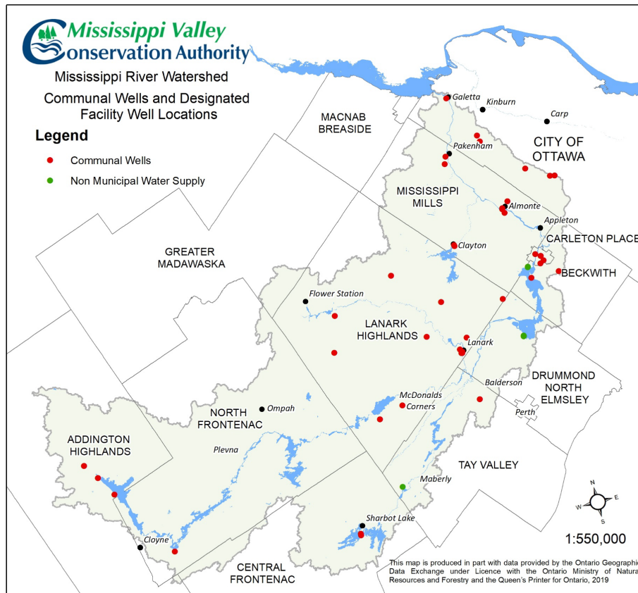
Figure 7: Known Communal Wells
