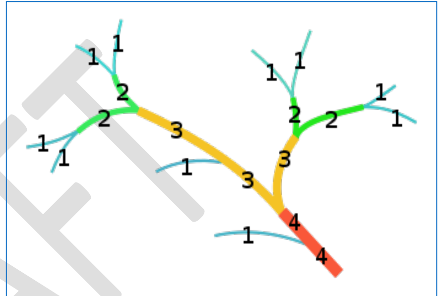
Figure 11: Strahler Stream Order Classification
