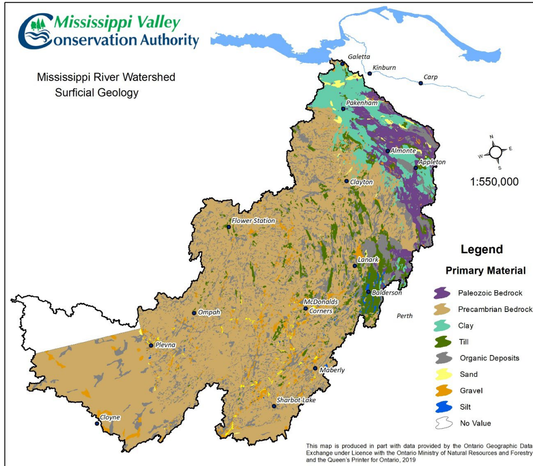
Figure 4: Surficial Geology
