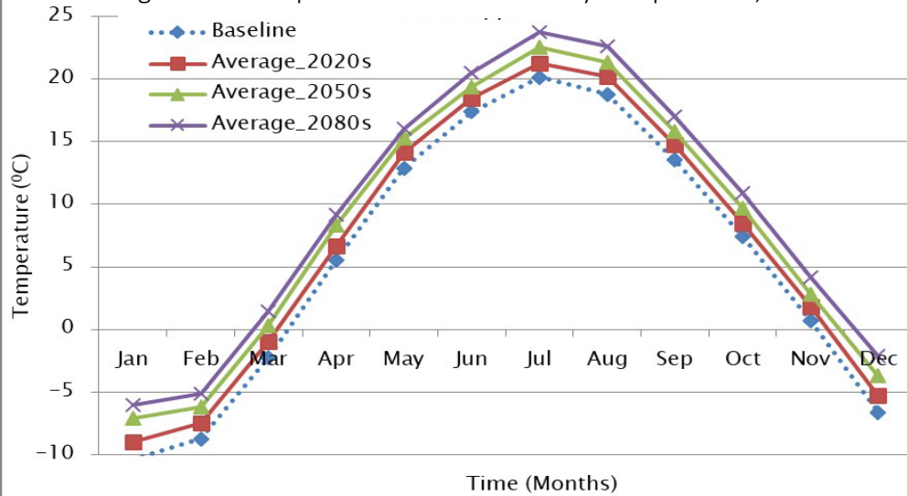
Figure 10: Comparison of Mean Monthly Temperature, 2010 to 2100
