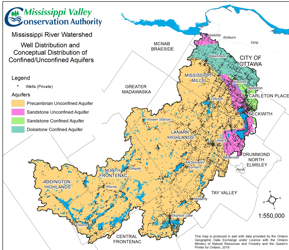
Figure 6: Well Distribution and Conceptual Distribution of Aquifers
