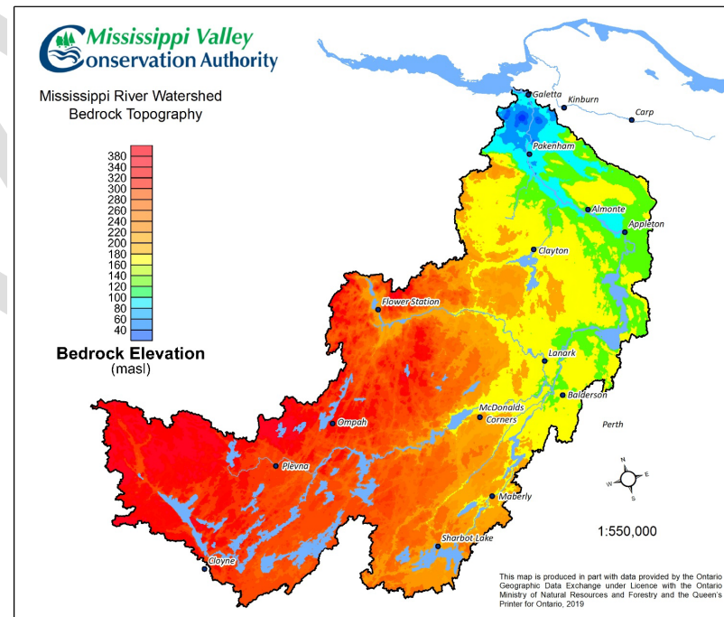
Figure 2: Bedrock Surface Topography
