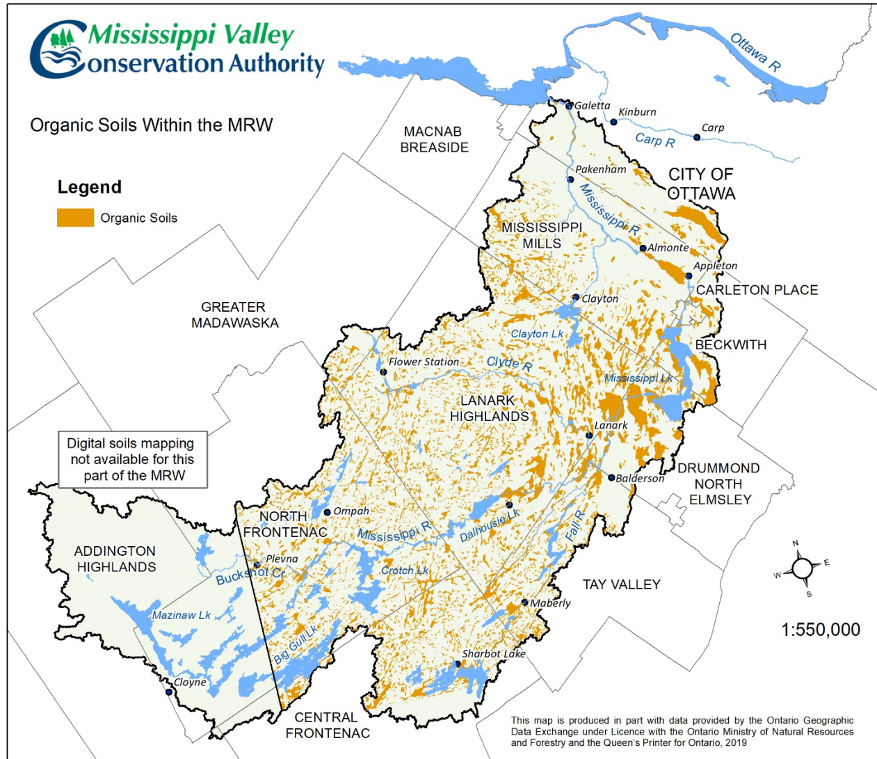
Figure 15: Organic Soils in the Mississippi River Watershed
