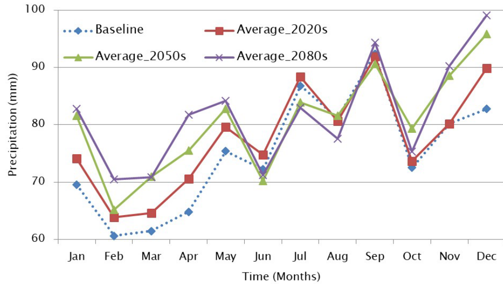
Figure 9: Comparison of Mean Monthly Precipitation, 2010 to 2100
