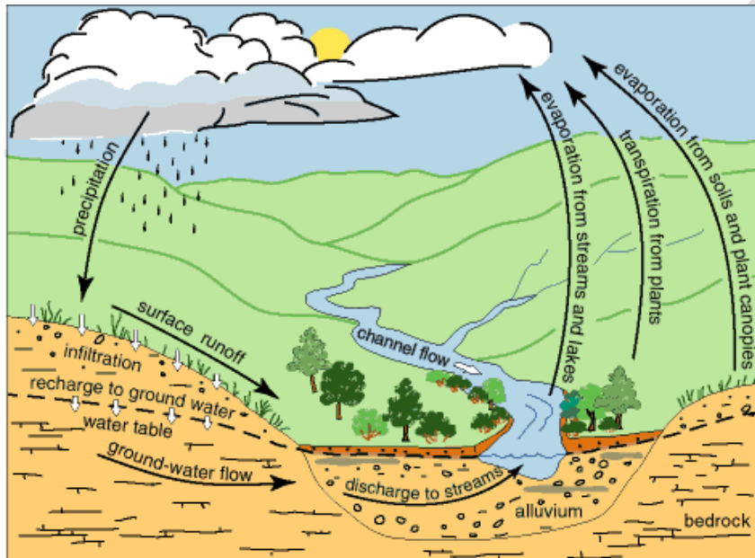
Figure 7: Water Cycle (Source: Kansas Geological Survey)
