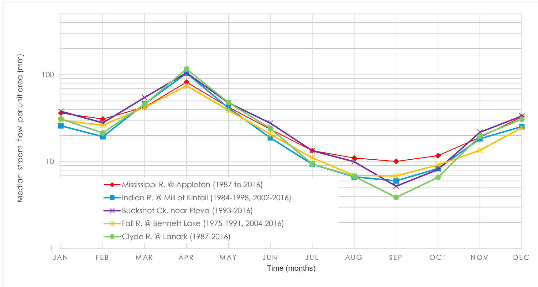
Figure 13: Median Stream Flow per Unit Area
