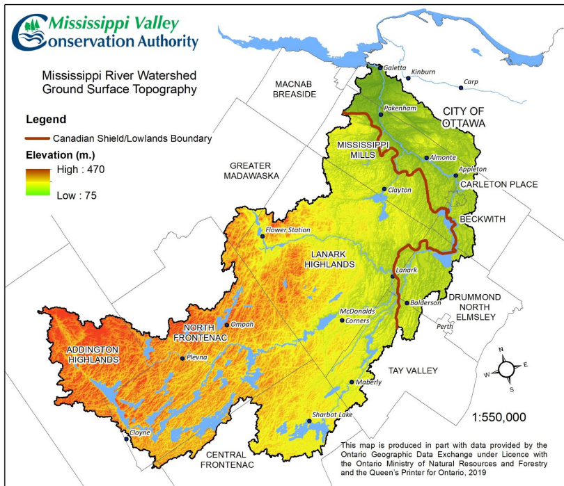
Figure 1: Ground Surface Topography
