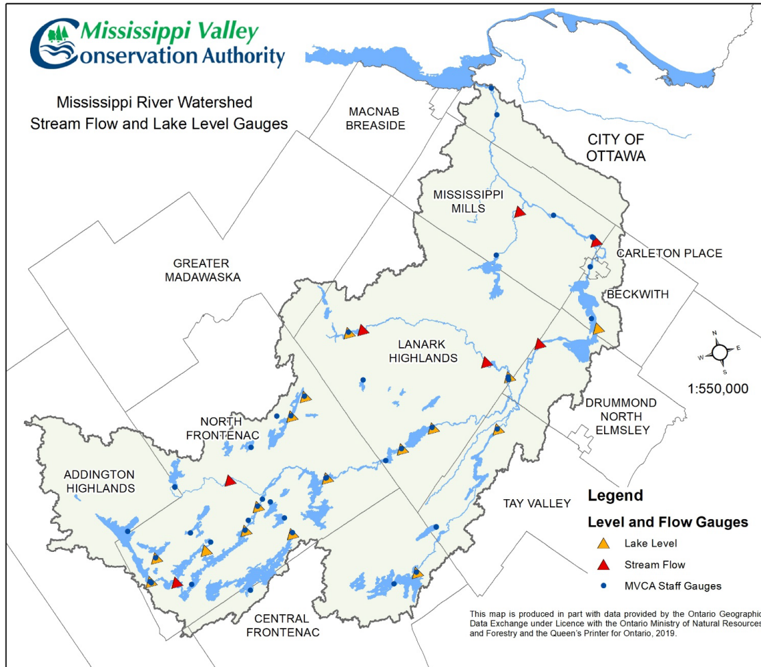
Figure 14: Water Level and Flow Gauges
