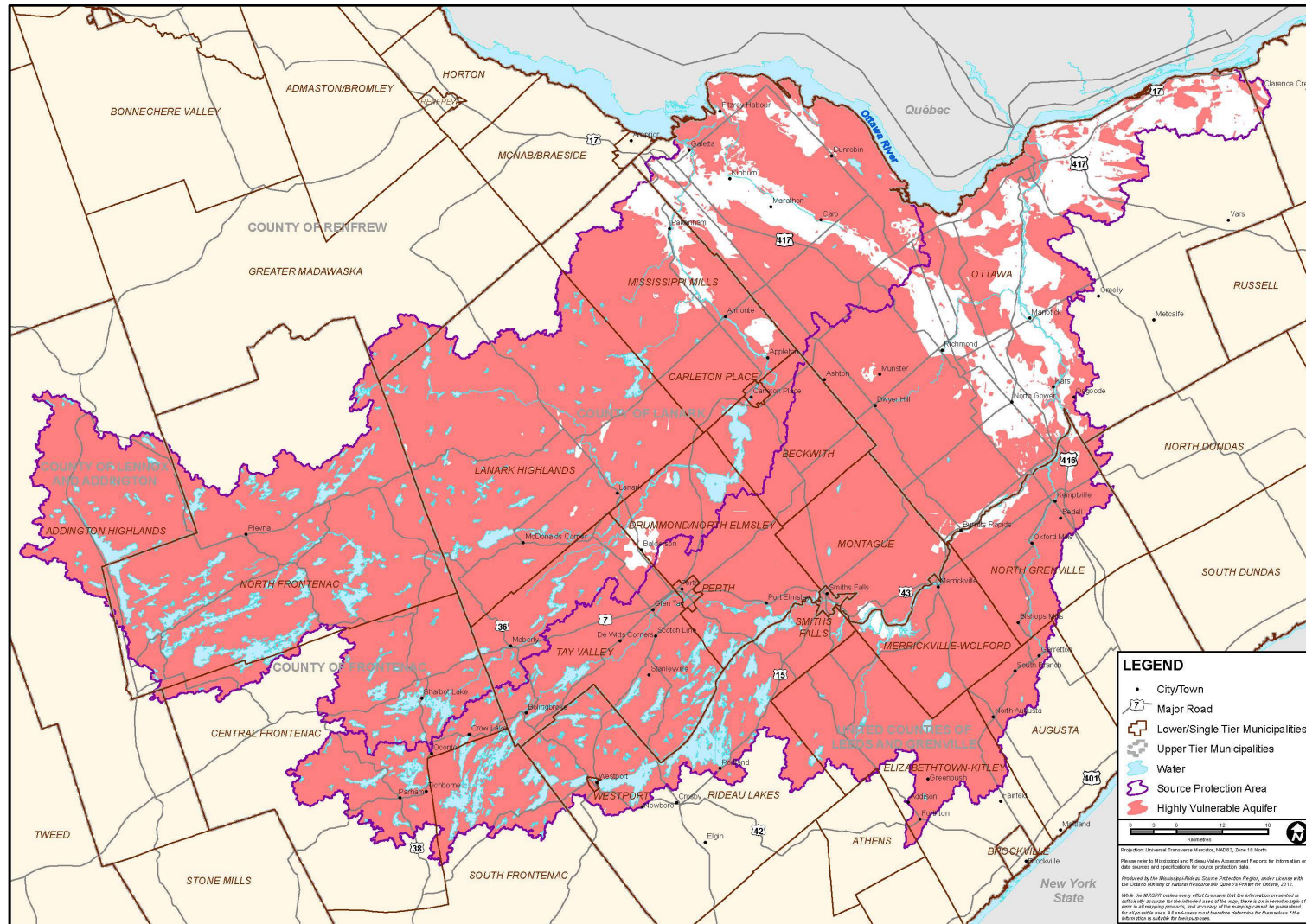
Figure 8: Highly Vulnerable Aquifer
