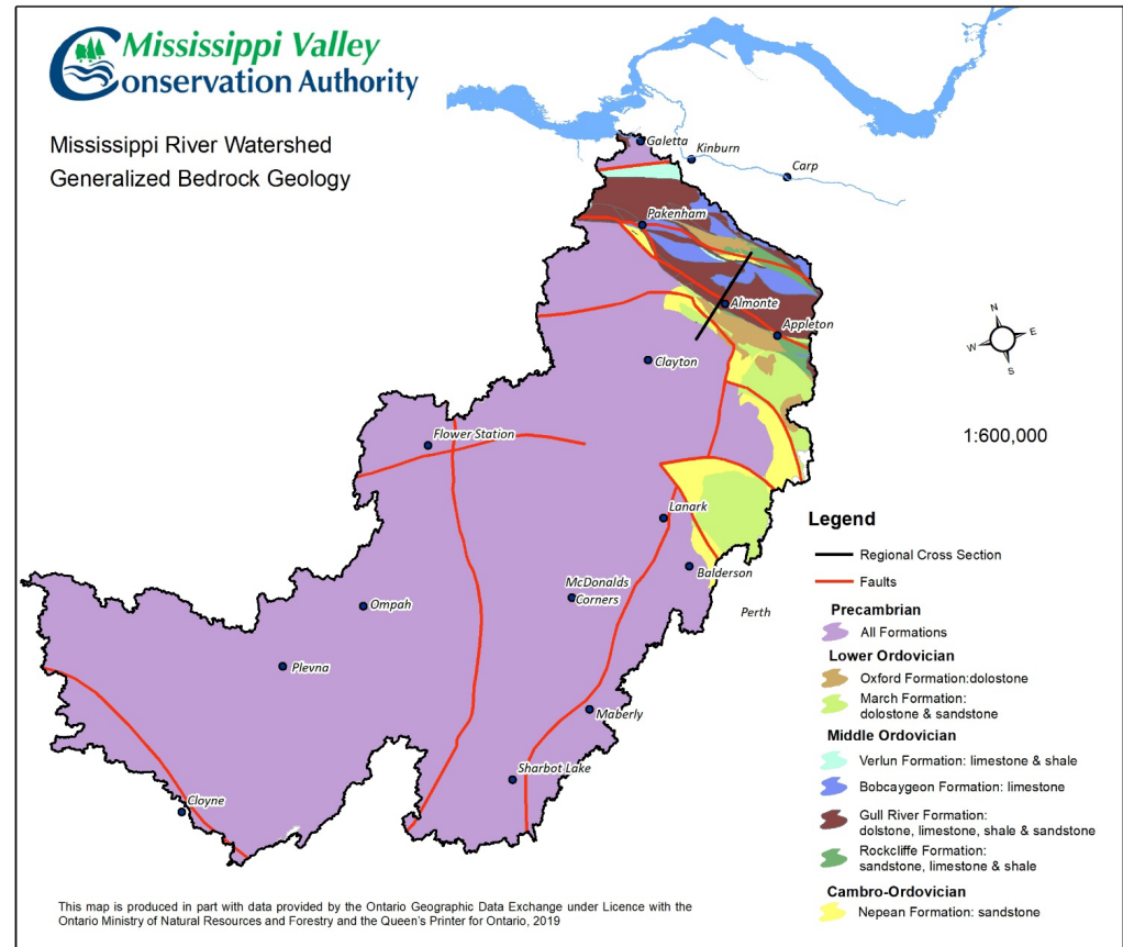
Figure 3: Generalized Bedrock Geology
