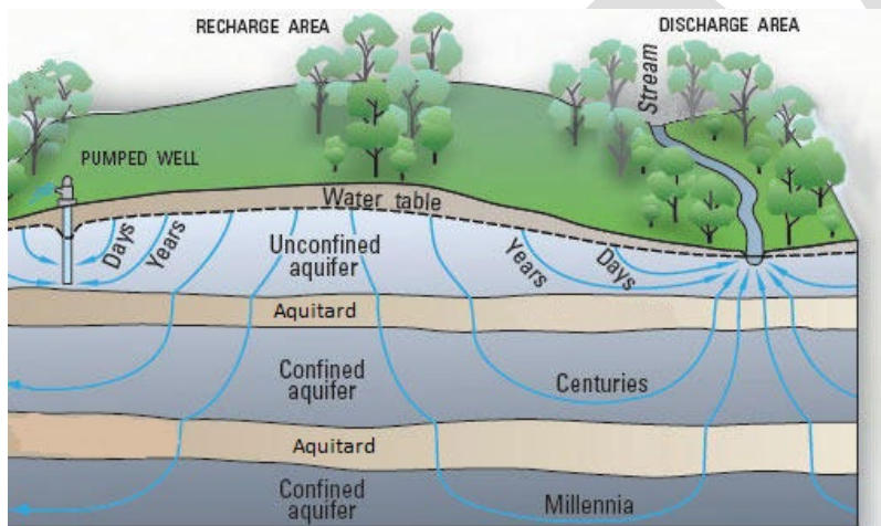
Figure 5: Conceptualized Diagram showing Aquifers and Aquitards
