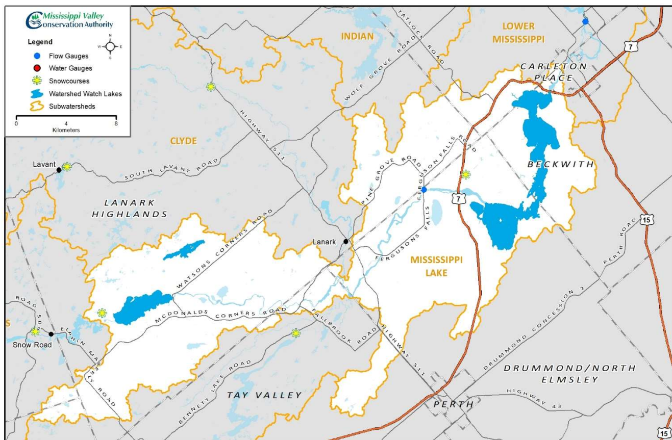
Figure 1: The various water quantity monitoring sites in the Mississippi Lake subwatershed, plus the lakes within the subwatershed that were monitored in 2021.
