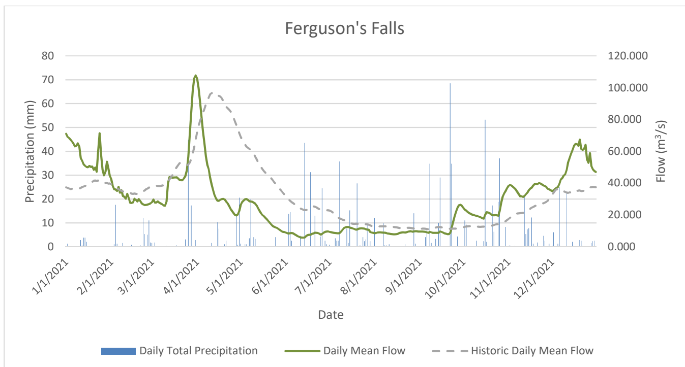
Figure 3c: Daily total precipitation and daily mean water flows at the Ferguson's Falls gauge station for 2021 compared to the historic daily mean flows for the site.
