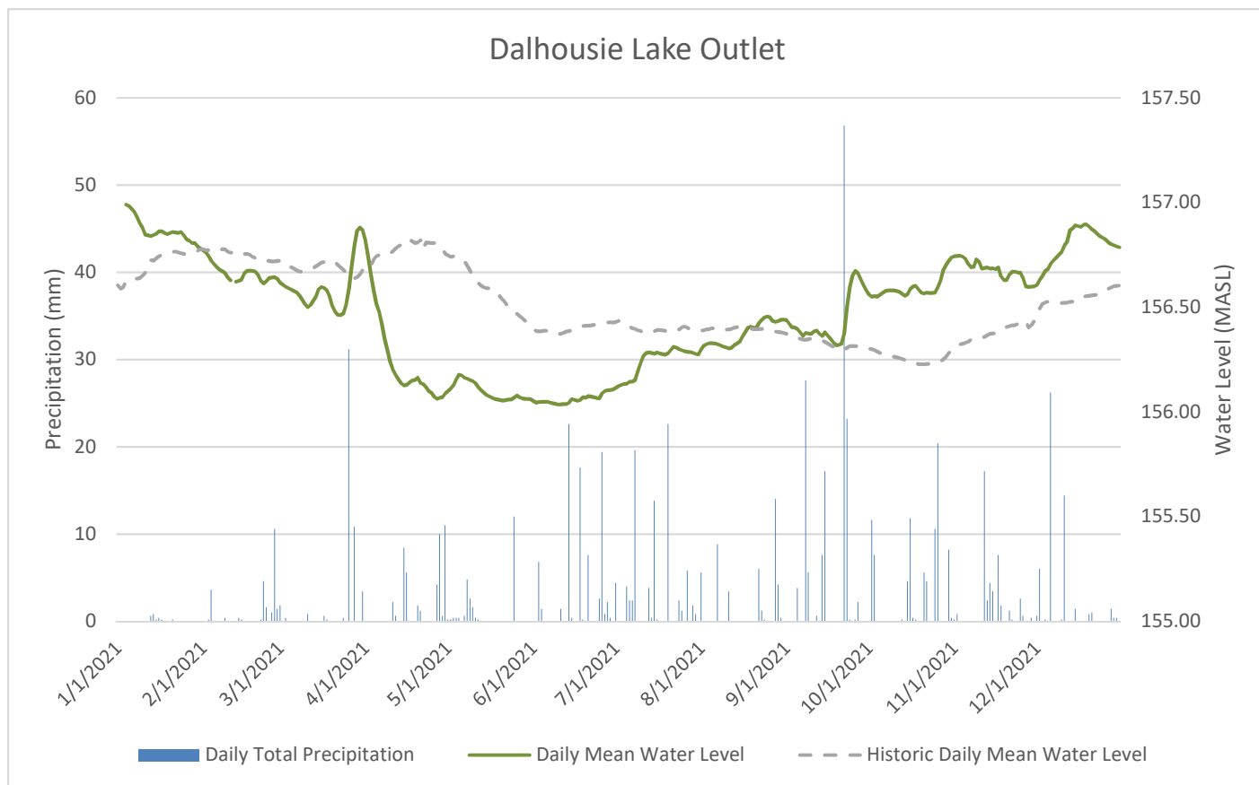
Figure 4c: 2021 and historic daily mean water levels (meters above sea level - MASL) at the Dalhousie Lake gauge compared to the 2021 daily total precipitation at the same gauge.
