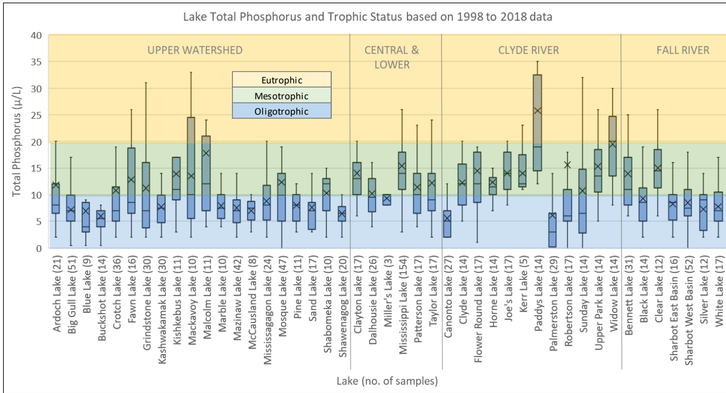
Figure 7: Lake Total Phosphorus and Trophic Status Ranges
