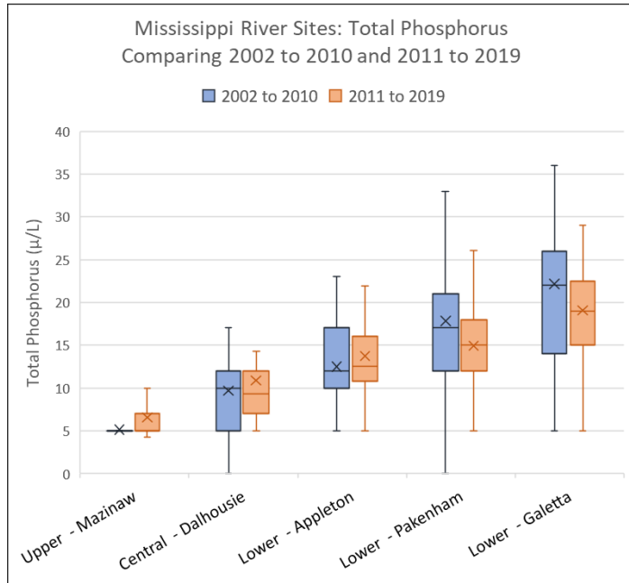
Figure 9: Mississippi River - Total Phosphorus
