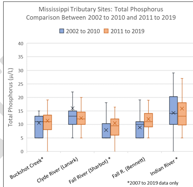
Figure 8: Mississippi Tributaries - Total Phosphorus
