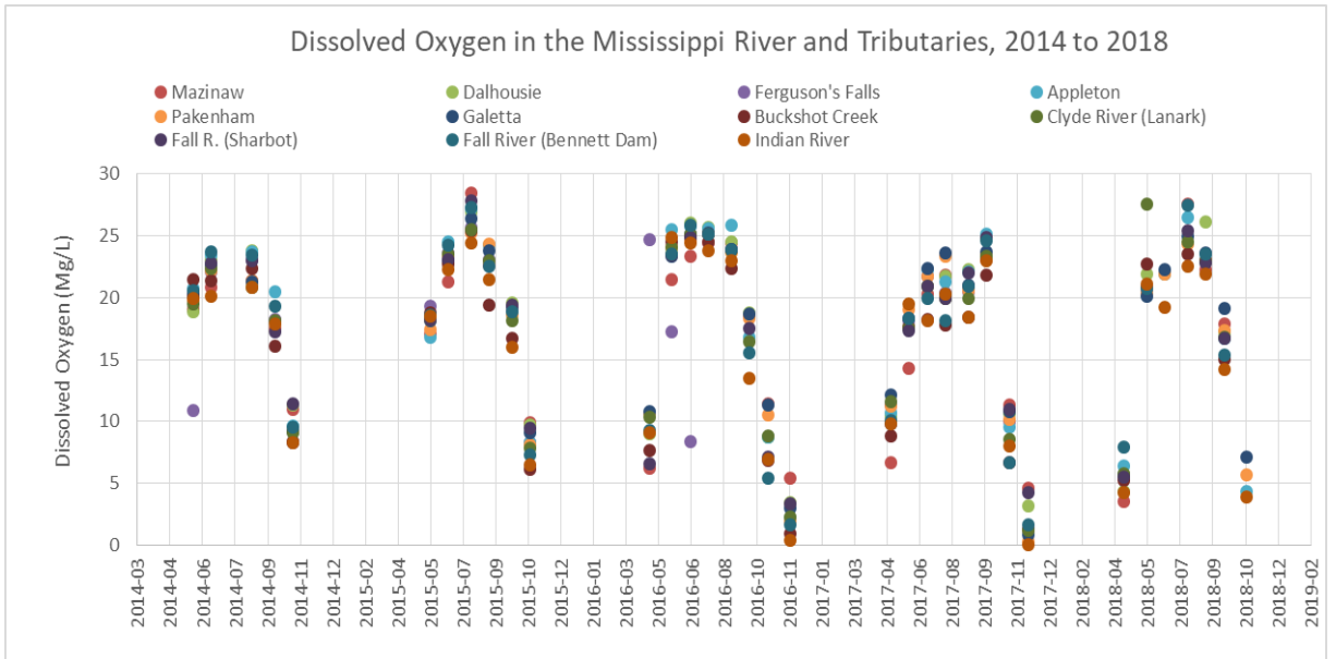
Figure 21: Dissolved Oxygen in the Mississippi River and Tributaries
