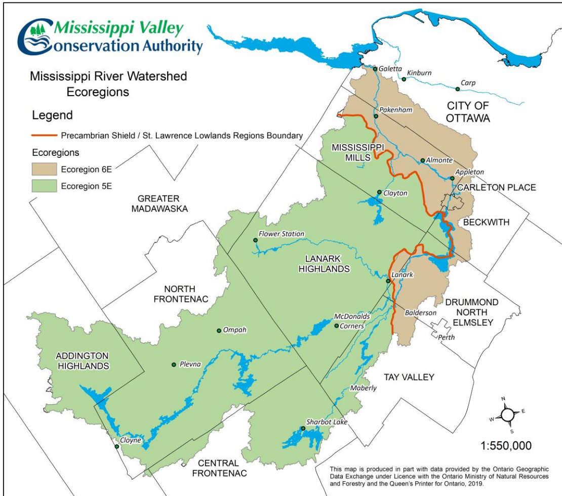
Figure 2: Ecoregions in the Mississippi River Watershed
