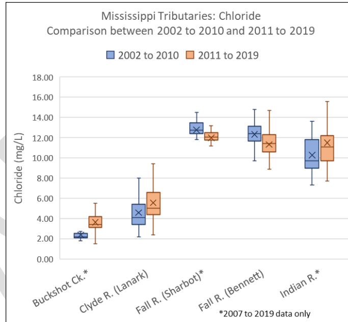
Figure 19: Mississippi Tributaries - Chloride
