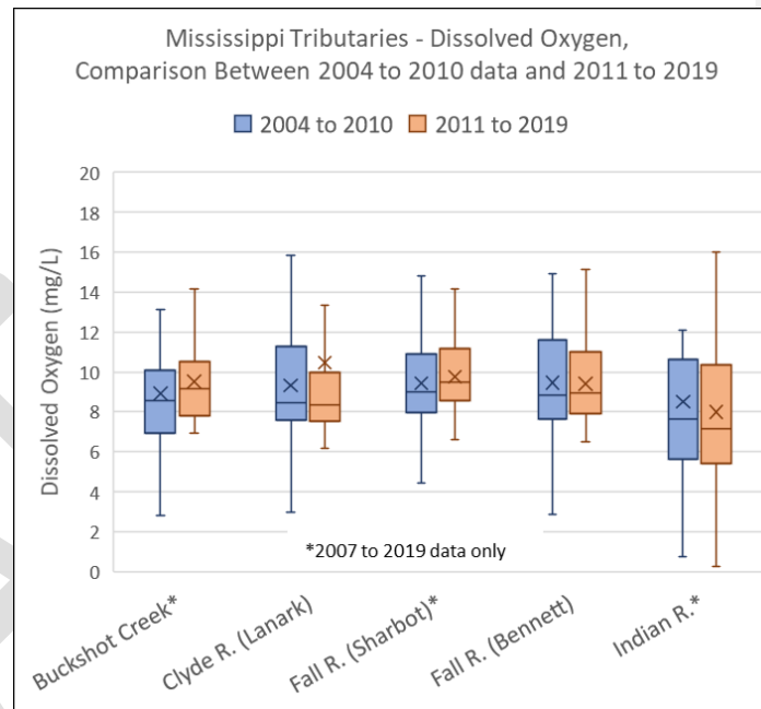
Figure 15: Mississippi Tributaries - Dissolved Oxygen
