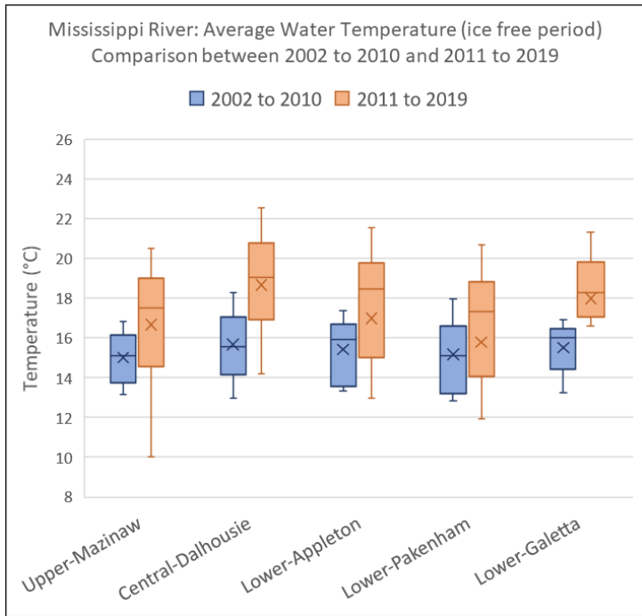
Figure 13: Mississippi River - Average Water Temperature
