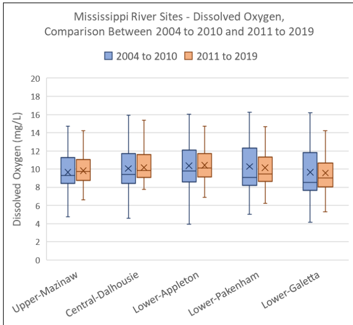
Figure 14: Mississippi River- Dissolved Oxygen
