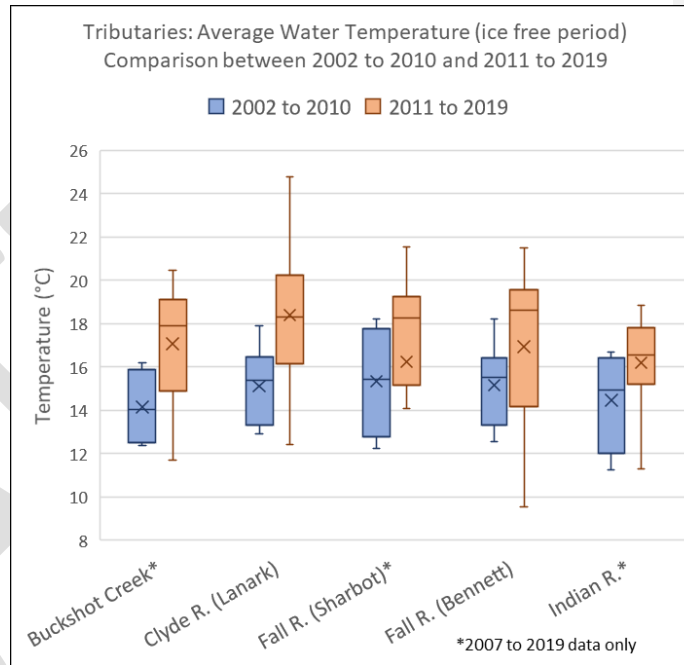
Figure 12: Mississippi Tributaries - Average Water Temperature
