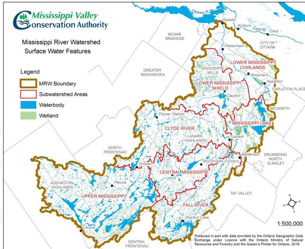
Figure 1: Mississippi River Watershed and Subwatersheds
