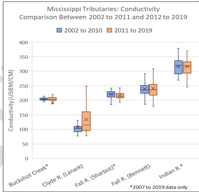
Figure 17: Mississippi Tributaries - Conductivity
