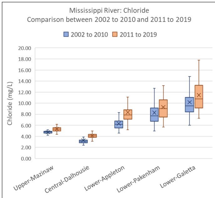
Figure 18: Mississippi River - Chloride
