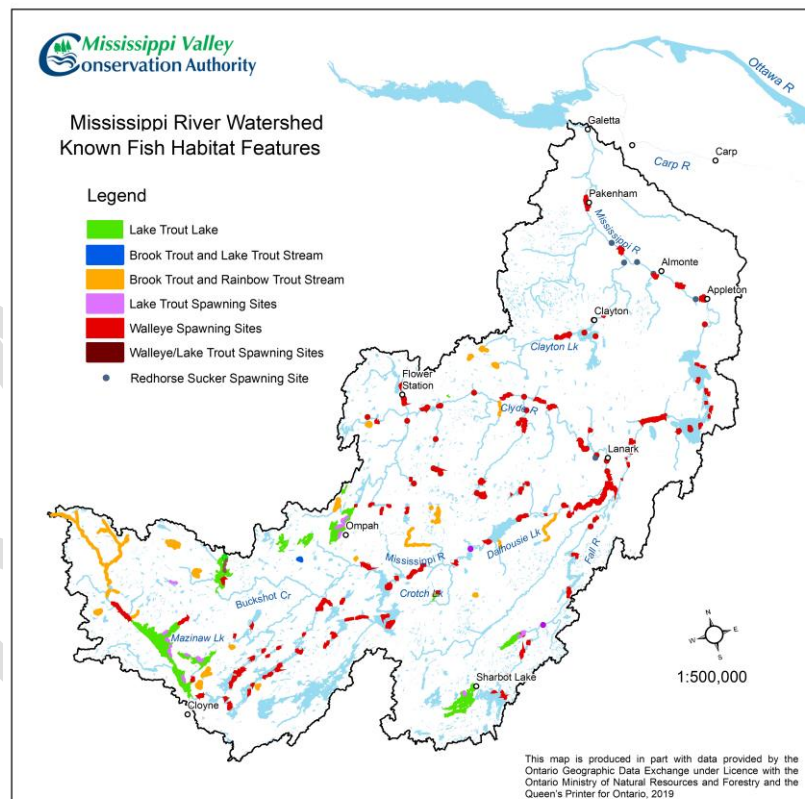
Figure 20: Known Fish Habitat Features
