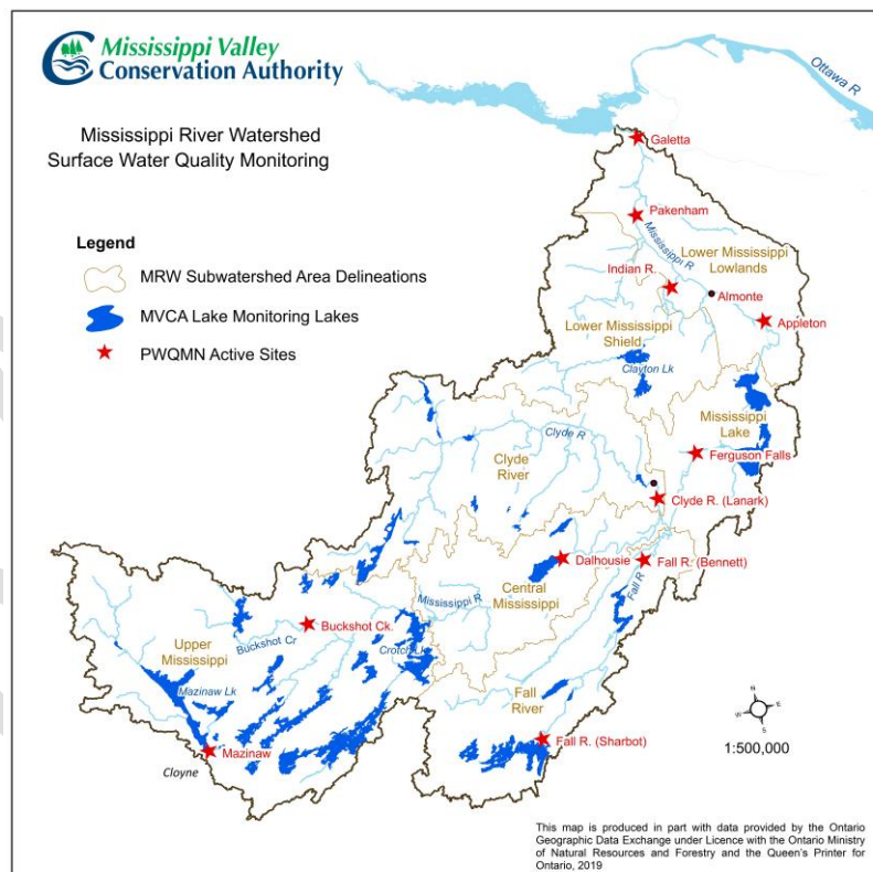
Figure 6: MVCA Lake Monitoring Sites and PWQMN Sites
