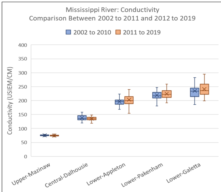
Figure 16: Mississippi River - Conductivity
