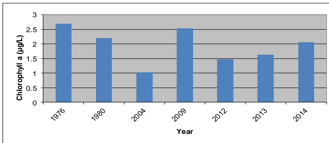
ARDOCH LAKE - MAIN BASIN ANNUAL MEAN CHLOROPHYLL a RESULTS (ug/L)
