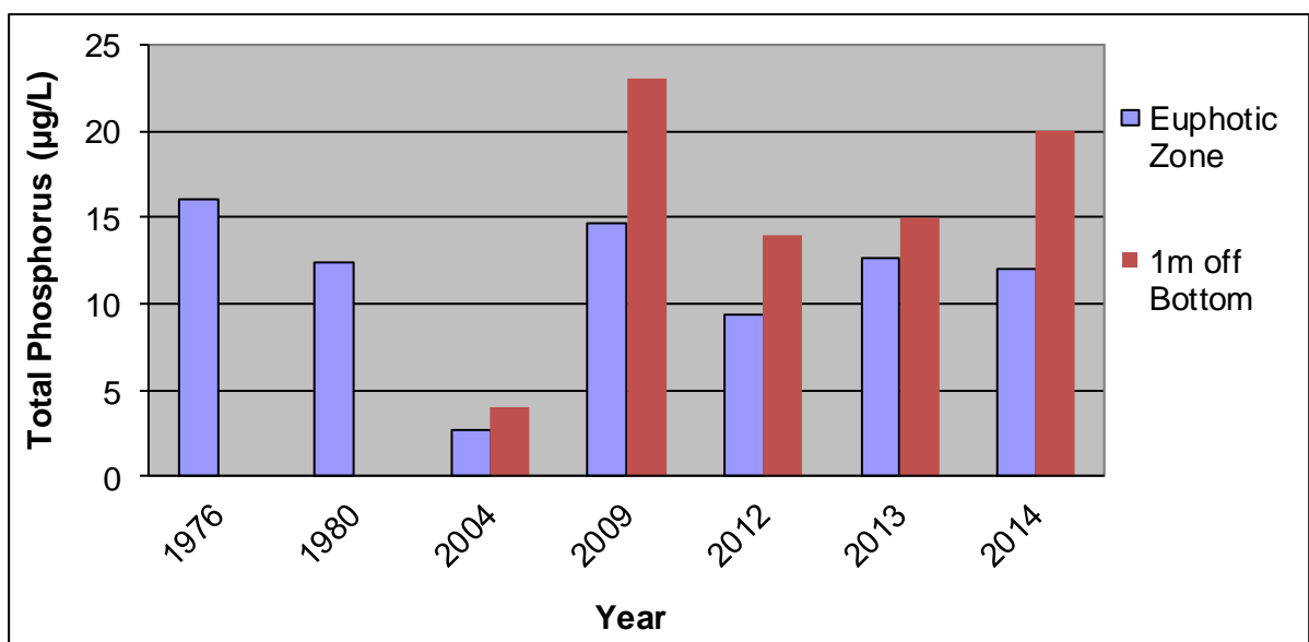
ARDOCH LAKE - MAIN BASIN ANNUAL MEAN TOTAL PHOSPHORUS RESULTS (ug/L)
