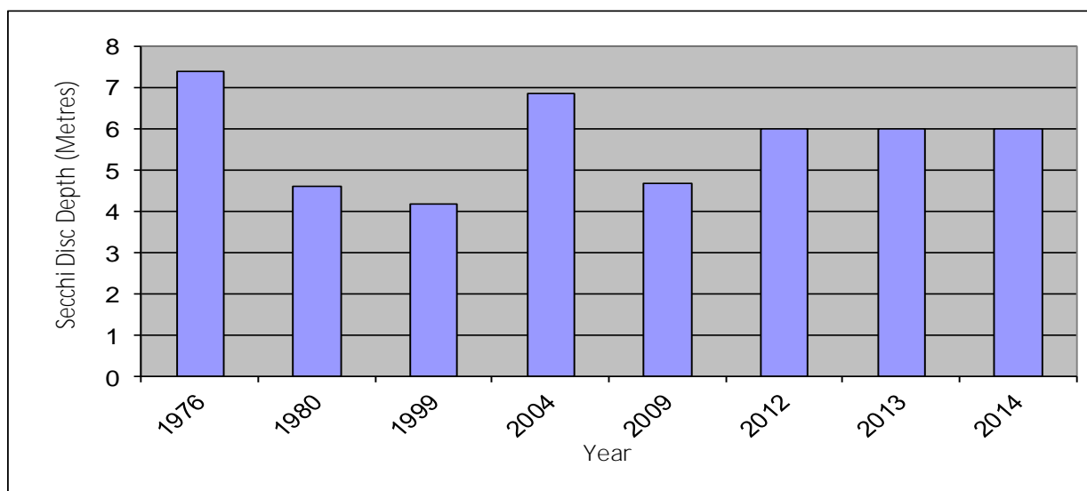
ARDOCH LAKE — MAIN BASIN ANNUAL MEAN SECCHI DISC DEPTHS (metres)
