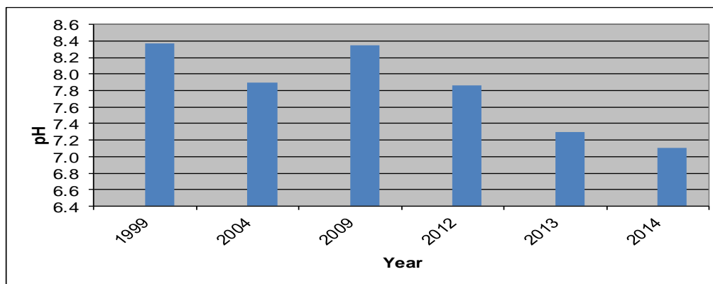
ARDOCH LAKE - MAIN BASIN pH LEVELS ALL YEARS
