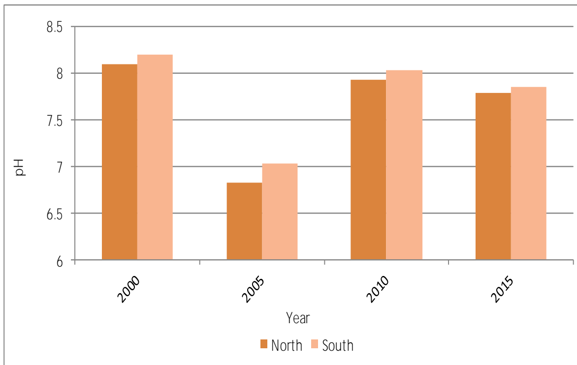
Grindstone Lake All Basins Annual Average pH
