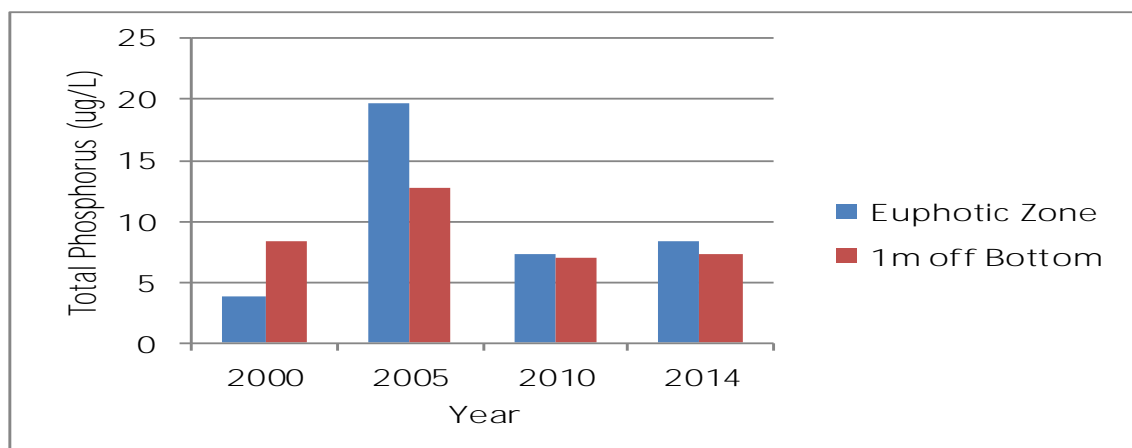
CROTCH LAKE - SOUTH BASIN ANNUAL MEAN TOTAL PHOSPHORUS RESULTS (ug/L)
