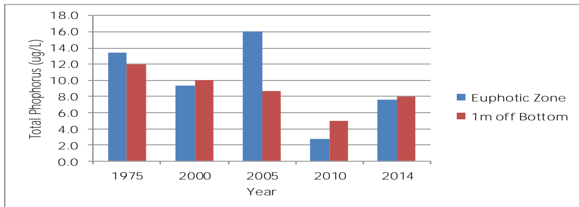
CROTCH LAKE - SOUTH BASIN ANNUAL MEAN TOTAL PHOSPHORUS RESULTS (ug/L)
