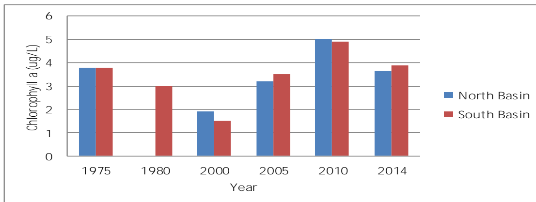
CROTCH LAKE - ALL BASINS ANNUAL MEAN CHLOROPHYLL a RESULTS (ug/L)
