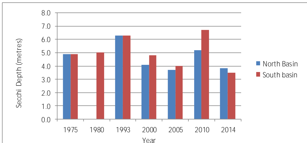
CROTCH LAKE — ALL BASINS ANNUAL MEAN SECCHI DISC DEPTHS (metres)
