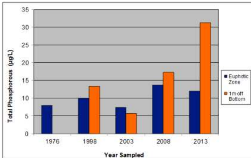
KISHKEBUS LAKE - MAIN BASIN ANNUAL MEAN TOTAL PHOSPHORUS RESULTS (ug/L)
