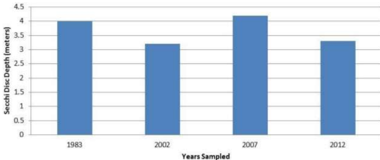
HORNE LAKE — MAIN BASIN ANNUAL MEAN SECCHI DISC DEPTHS (metres)
