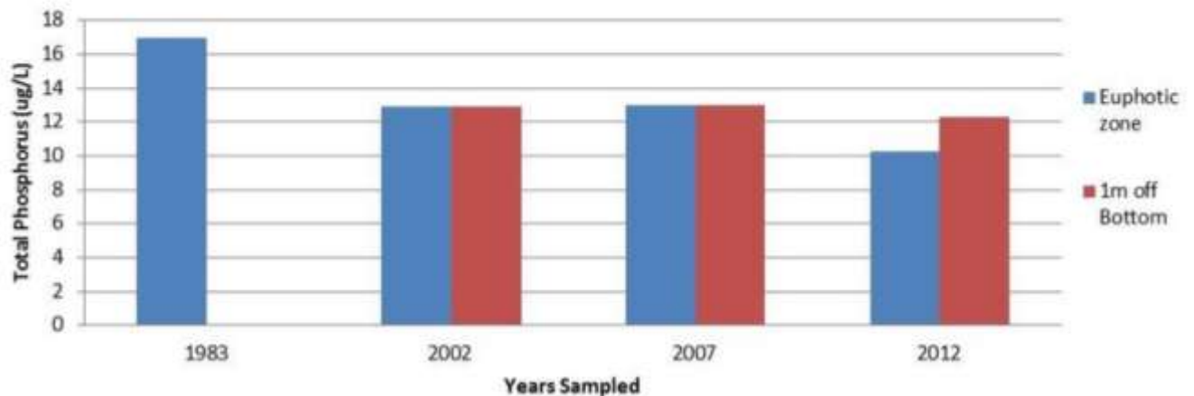
HORNE LAKE - MAIN BASIN ANNUAL MEAN TOTAL PHOSPHORUS RESULTS (ug/L)
