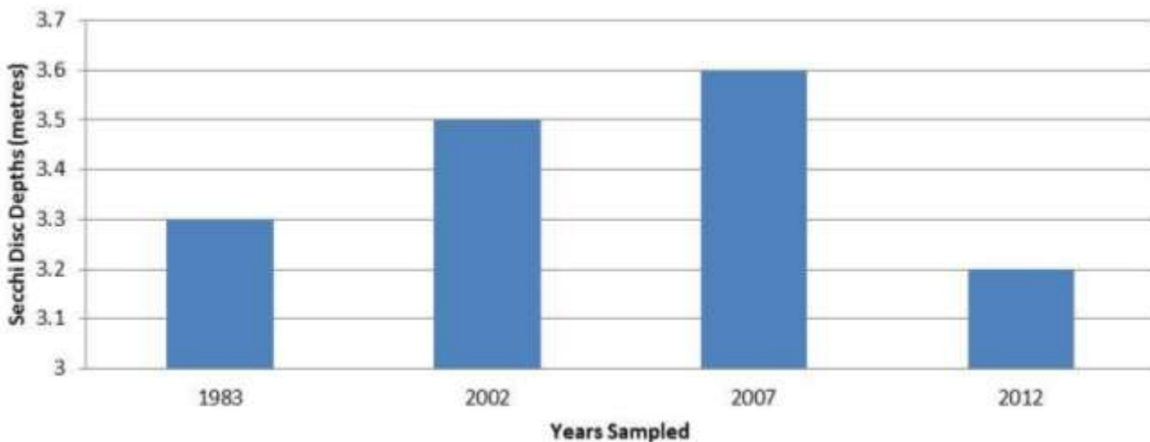
CLYDE LAKE — MAIN BASIN ANNUAL MEAN SECCHI DISC DEPTHS (metres)
