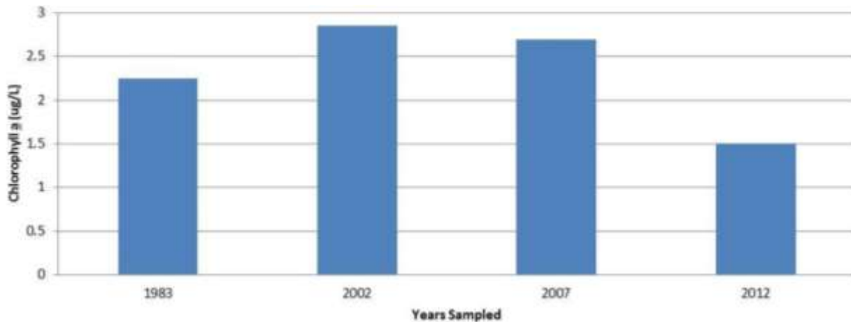
CLYDE LAKE - MAIN BASIN ANNUAL MEAN CHLOROPHYLL a RESULTS (ug/L)
