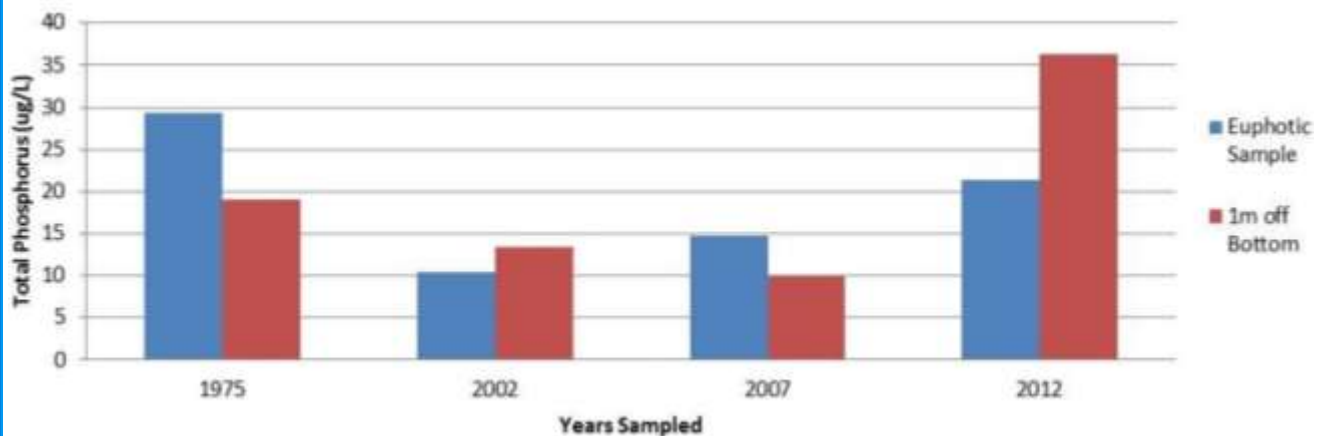
CLAYTON LAKE - MAIN BASIN ANNUAL MEAN TOTAL PHOSPHORUS RESULTS (ug/L)
