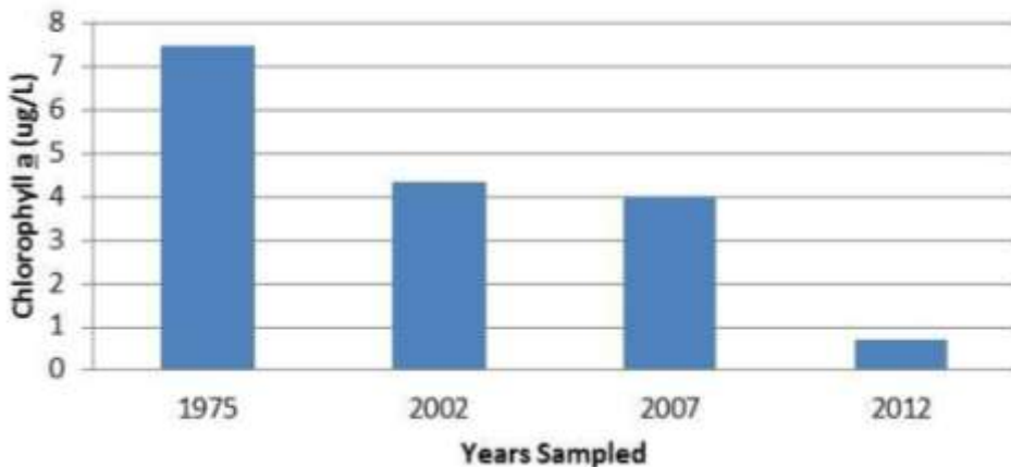
CLAYTON LAKE - MAIN BASIN ANNUAL MEAN CHLOROPHYLL a RESULTS (ug/L)
