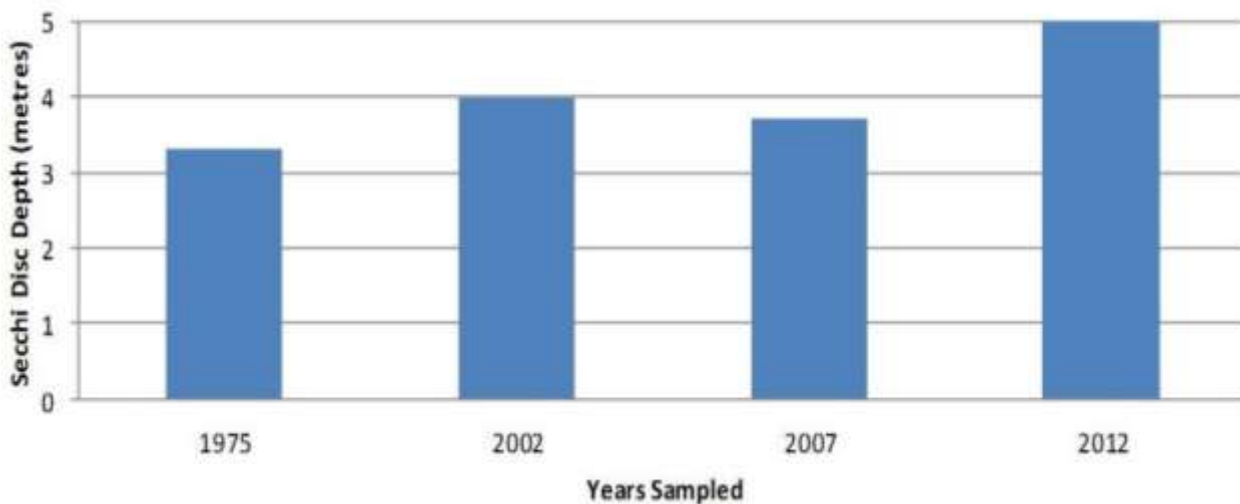
CLAYTON LAKE — MAIN BASIN ANNUAL MEAN SECCHI DISC DEPTHS (metres)
