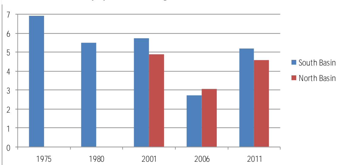
Bennett Lake—South and North Basins Annual Mean Chlorophyll a Results (ug/L)
