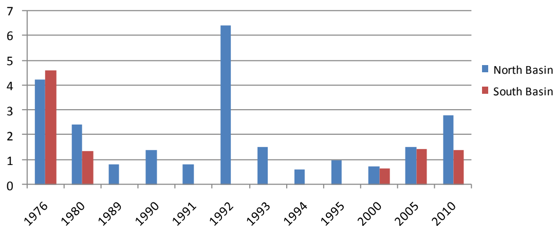
Canonto Lake—North and South Basins Annual Mean Chlorophyll a Results (ug/L)
