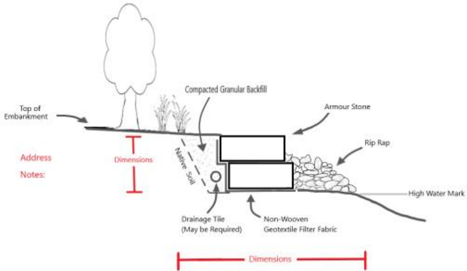
Conceptual Drawing of Armour Stone Retaining Wall Cross-Sectional View
