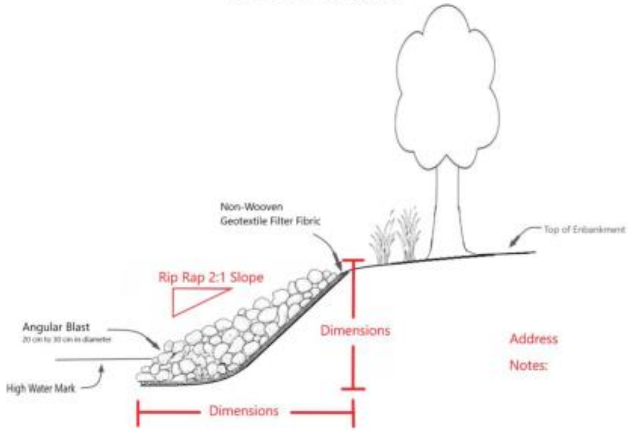
Conceptual Drawing of Rip Rap Erosion Protection Cross-Sectional View
