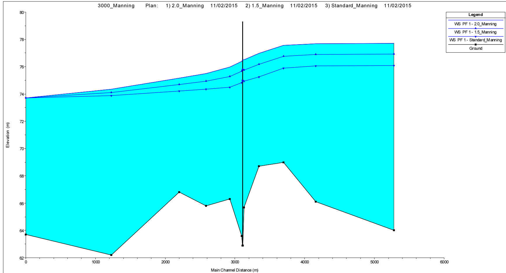
Figure E1 – Manning’s n Sensitivity Analysis 1:100 Year Water Surface for Sections 3011 to 3001
