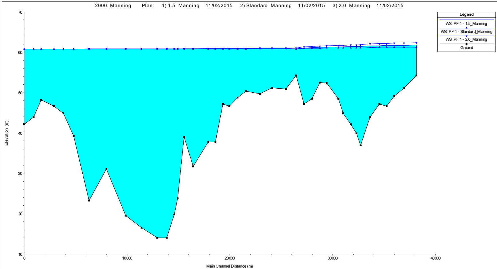
Figure E2 – Manning’s n Sensitivity Analysis 1:100 Year Water Surface for Sections 2059 to 2019
